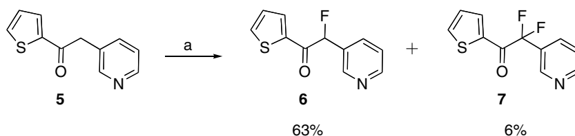
Scheme 1. Reagents and conditions: (a) LiHMDS (1.05 equivalent), NFSi (1.1 equivalent), THF, -78^\circ\text{C} , 4 h.
