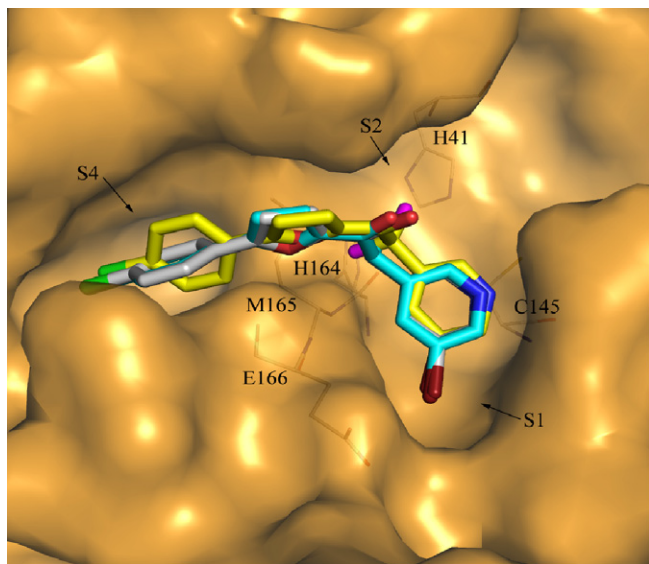
Fig. 2. The modeled binding conformations of 11d (white carbon sticks), 12d (cyan carbon sticks) and 13d (yellow carbon sticks) in the active site of SARS-CoV 3CL pro (oxygen atoms are red; nitrogen atoms are blue; chlorine atoms are green; bromine atoms are maroon; and fluorine atoms are purple).
