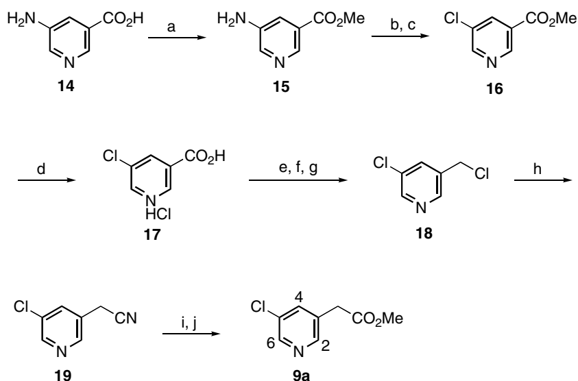
Scheme 3. Reagents and conditions: (a) MeOH, SOCl 2 , reflux, 8 h, 88%; (b) NaNO 2 , Conc. HCl, 0 °C, 1 h; (c) 10% HCl, CuCl, CuCl 2 , 0 °C, 4 h, 79%; (d) KOH, MeOH/H 2 O, rt, 24 h, 84%; (e) Et 3 N, EtOCOCl, 0 °C, 1.5 h; (f) LiAlH 4 , −78 °C, 4 h; (g) SOCl 2 , rt, 42 h, 76%; (h) KCN, DMF, rt, 48 h, 56%; (i) Conc. HCl, H 2 O, reflux, 12 h; (j) MeOH, SOCl 2 , reflux, 8 h, 72%.
