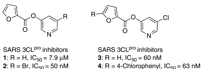
Fig. 1. Pyridinyl esters 1–4 as potent SARS 3CL pro inhibitors.
