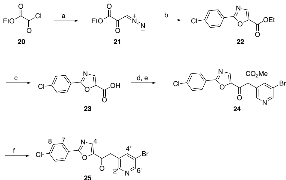
Scheme 4. Reagents and conditions: (a) TMSCHN 2 , THF, rt, 3 h, 68%; (b) 4-chlorobenzonitrile, Cu(acac) 3 , benzene, reflux, 12 h, 14%; (c) LiOH, THF/H 2 O, 0 °C, 2 h; (d) CDI, THF, 1 h; (e) 9c , LiHMDS, THF, -78 °C, 4 h, 23%; (f) 50% aqueous H 2 SO 4 , reflux, 8 h, 58%.
