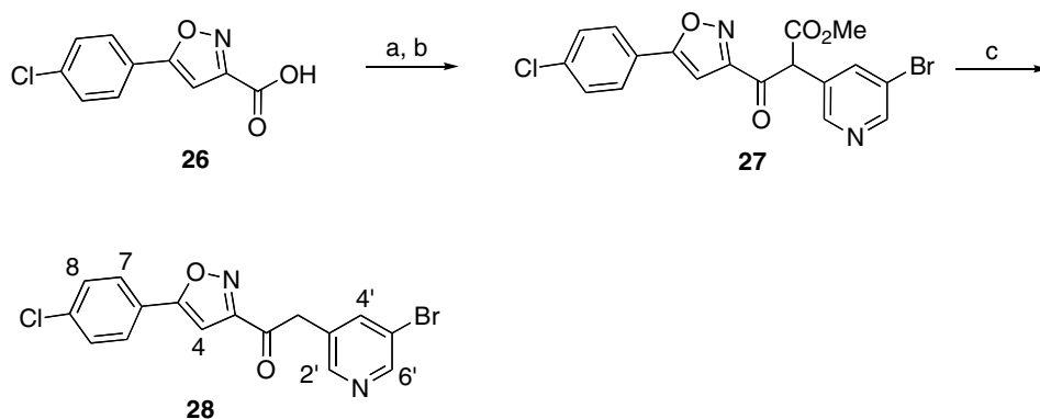
Scheme 5. Reagents and conditions: (a) CDI, THF, 1 h; (b) 9c , LiHMDS, THF, -78 °C, 4 h, 19%; (c) 50% aqueous H 2 SO 4 , reflux, 8 h, 58%.
