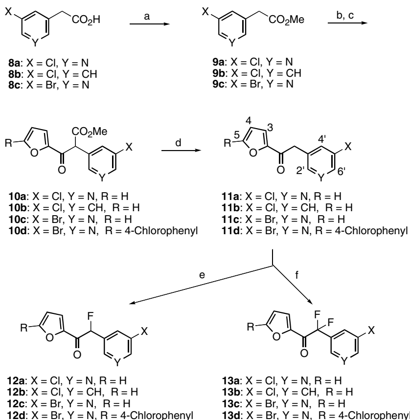
Scheme 2. Reagents and conditions: (a) MeOH, HCl, reflux, 12 h, 88%–quant.; (b) LiHMDS, THF, -78^{\circ}\text{C} , 1 h; (c) furan-2-carboxylic acid or 5-(4-chlorophenyl)furan-2-carboxylic acid, CDI, THF, 3 h, 72–96%; (d) 50% aqueous \text{H}_2\text{SO}_4 , reflux, 8 h, 59–85%; (e) LiHMDS (1.1 equivalent), NFSi (1.1 equivalent), THF, -78^{\circ}\text{C} , 4 h, 50–88%; (f) LiHMDS (2.2 equivalent), NFSi (2.2 equivalent), THF, -78^{\circ}\text{C} , 4 h, 34–85%.
